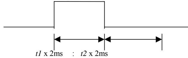
< Figure 3.2 Drawer Kick-out Drive Signal Output Waveform >
